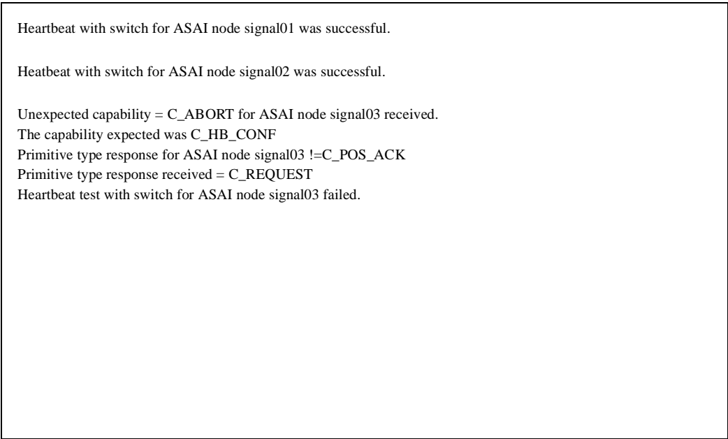
Screen 3-40. ASAI Test
