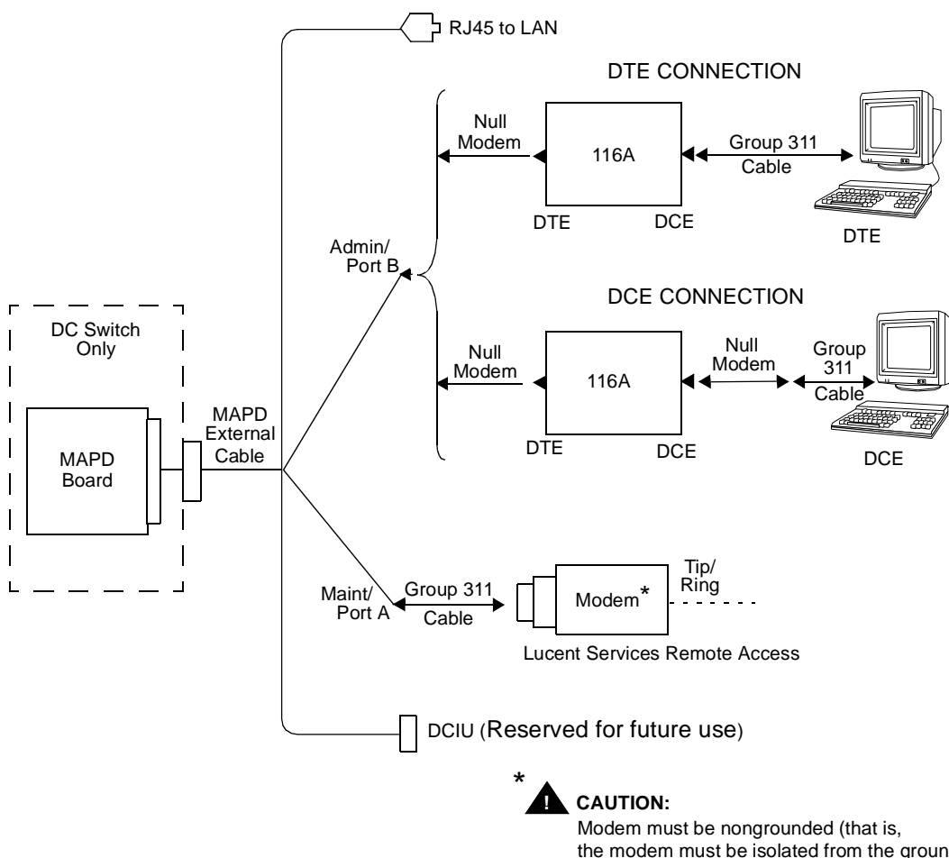
Figure 2-11. Installing a Terminal via Direct Connection (DC Switch Only)
