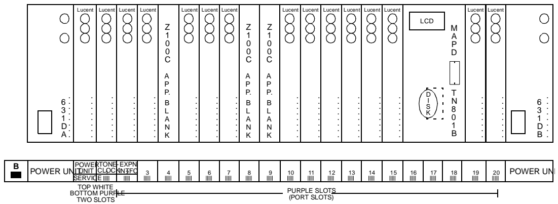
Figure 2-1. MAPD System in a DEFINITY System Carrier
